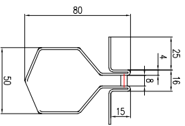
Channel profile M(1:1)
