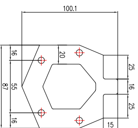
Flange for H80 M(1:1)
