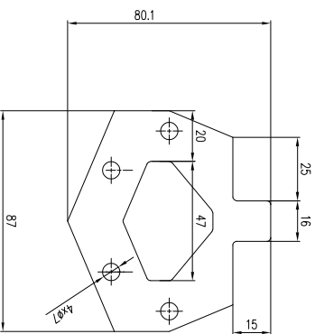
Flange for H60 M(1:1)
