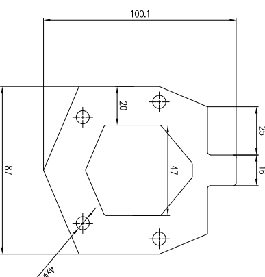
Flange for H80 M(1:1)
