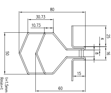
Channel profile M(1:1)
